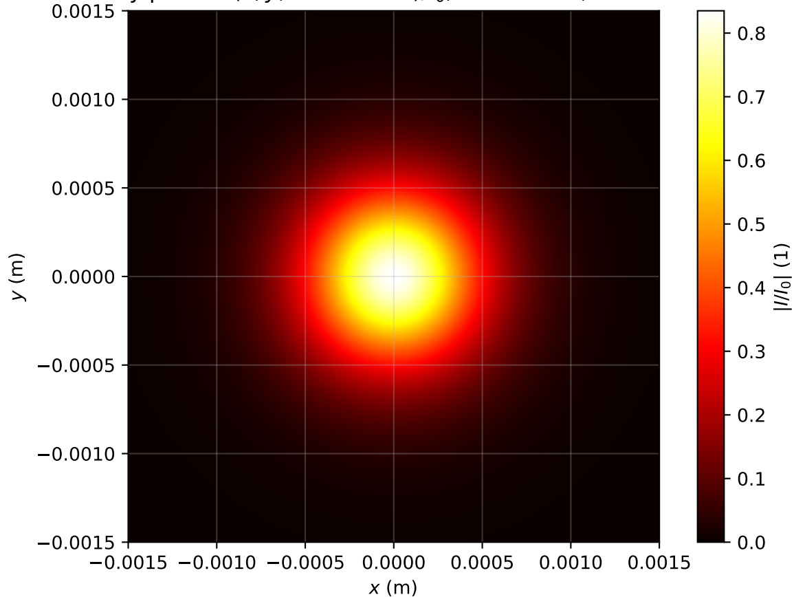
Intensity profile I(x, y, z = 2.388m)/I_0 , \text{Pin}=0.6\text{Pcr} , artificial time
